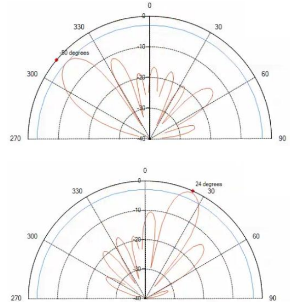
Beam forming radiation patterns
