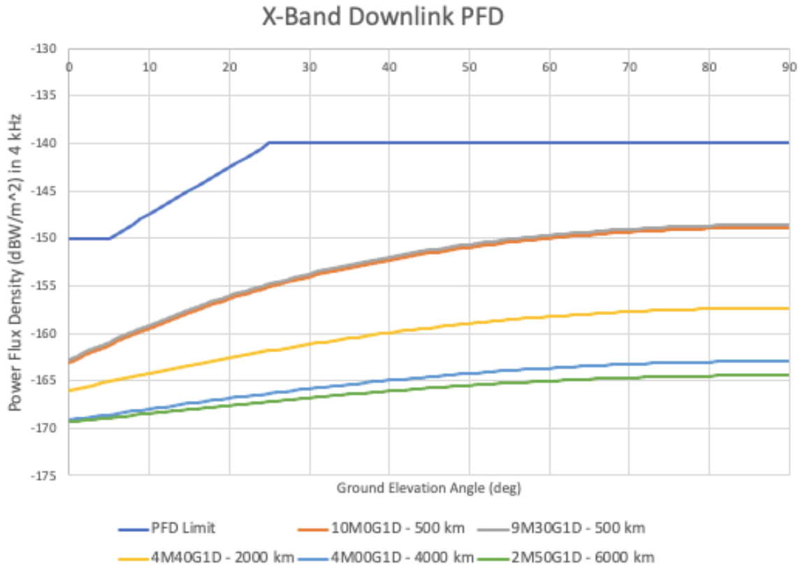
Figure 2. X-Band Power Flux Density at the surface of the Earth.
