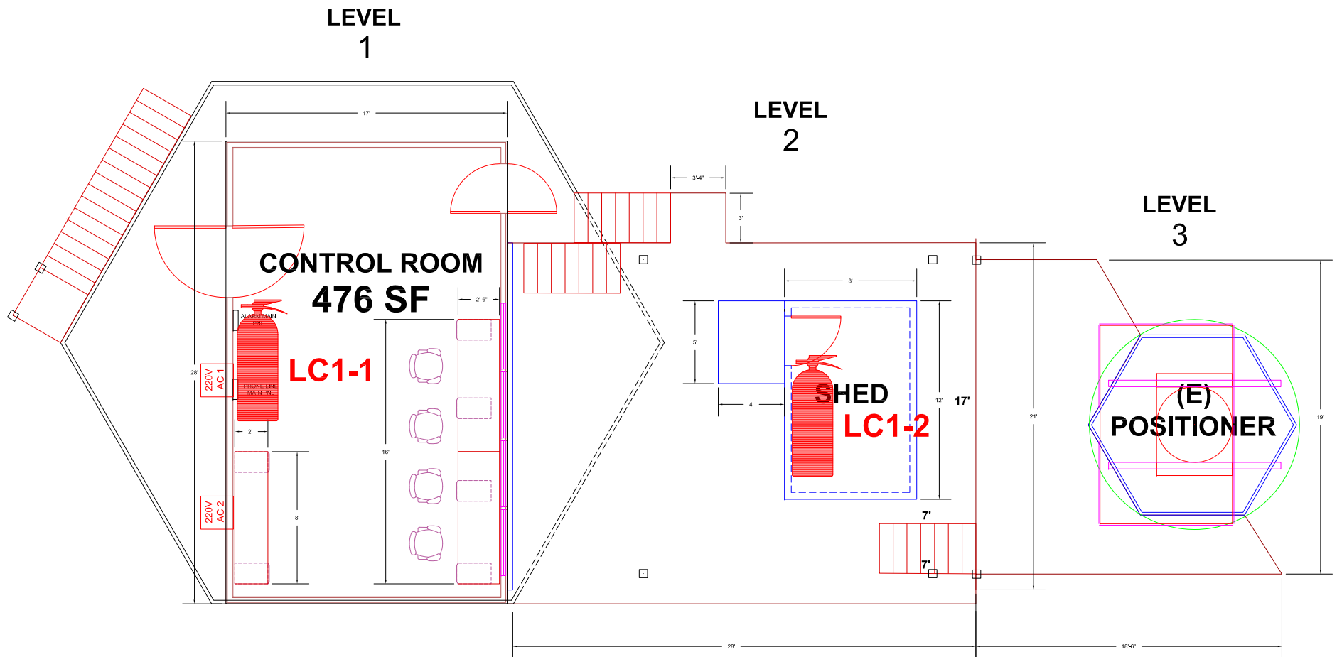
PLAN VIEW
