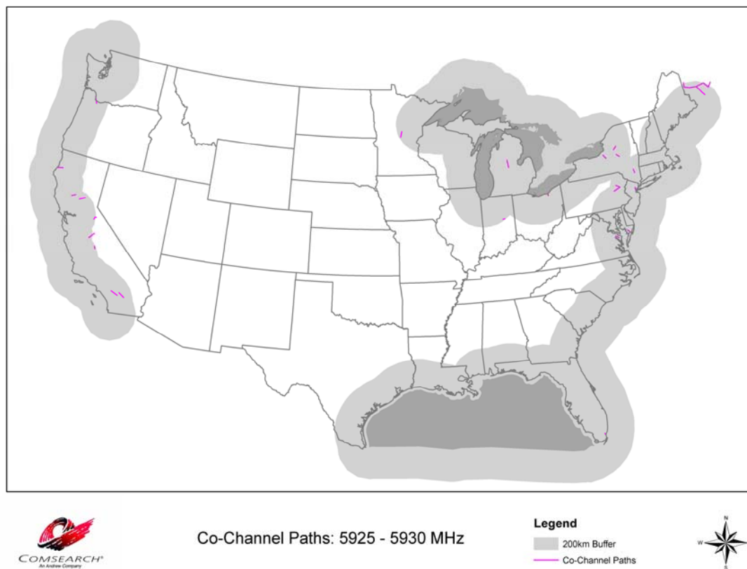
Figure 1 – Terrestrial Microwave Links with channels overlapping 5925-5930.0 MHz
