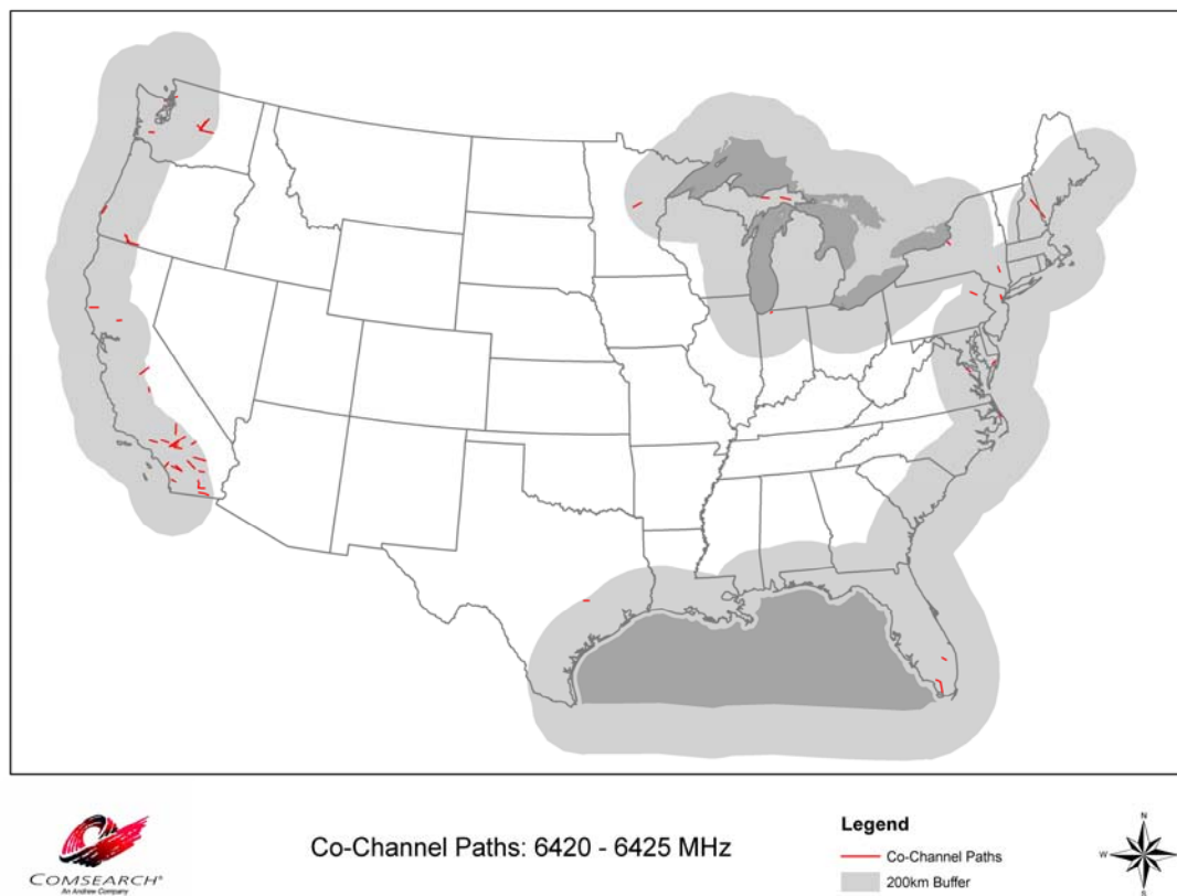
Figure 2 – Terrestrial Microwave Links with channels overlapping 6420.0-6425. MHz
