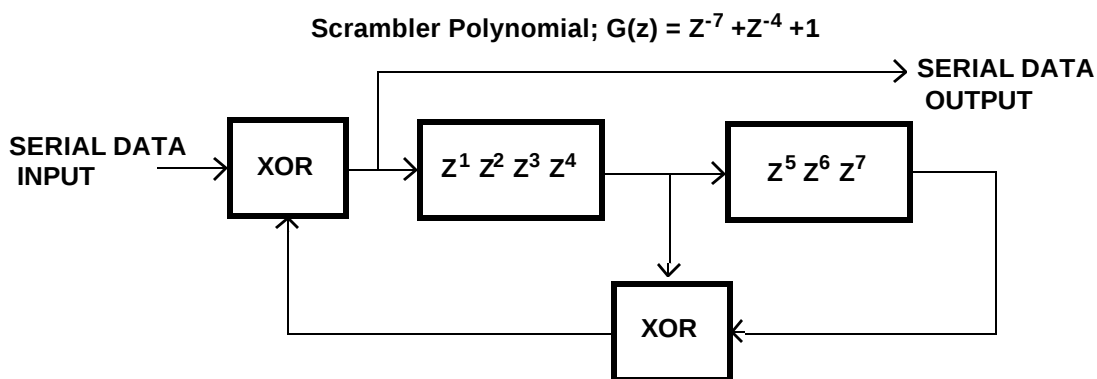
Figure 5—Data scrambler
