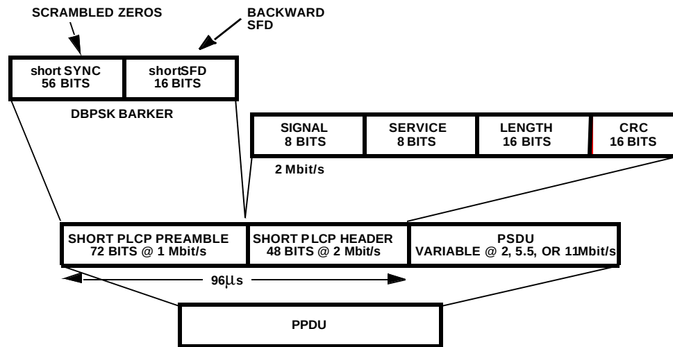
Figure 2—Short PLCP PDU format
