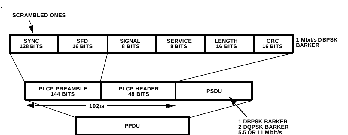
Figure 1—Long PLCP PPDU format
