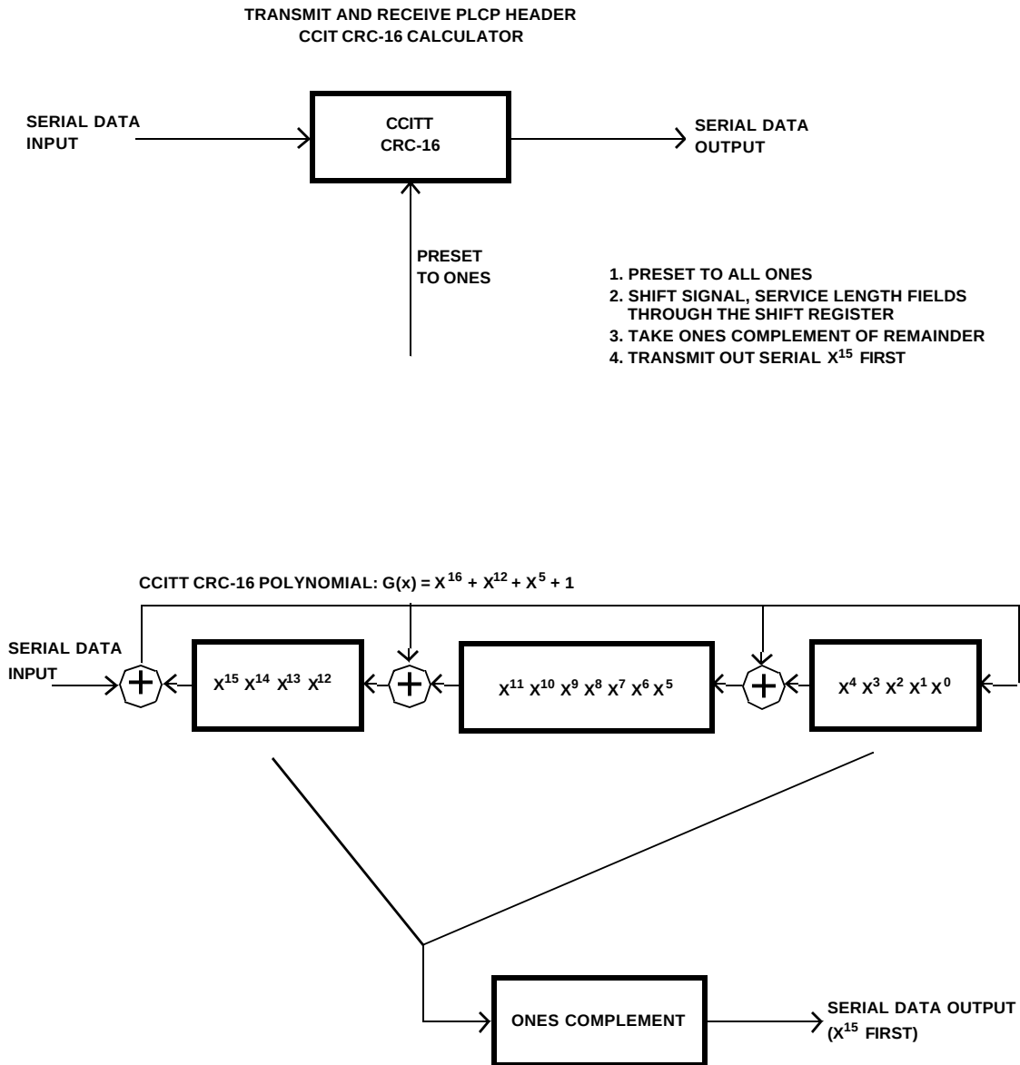
Figure 3—CCITT CRC-16 Implementation
