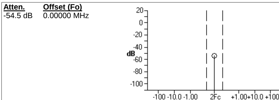
Figure 1 - 2nd Harmonic Curve (U)
