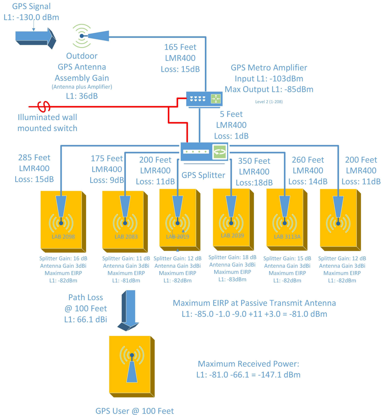
Figure 3 - GPS re-radiation system diagram
