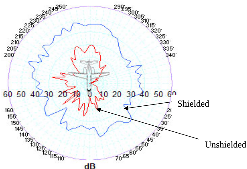
Figure 18. Relative attenuation Shielded Vs Unshielded 2435 MHz
