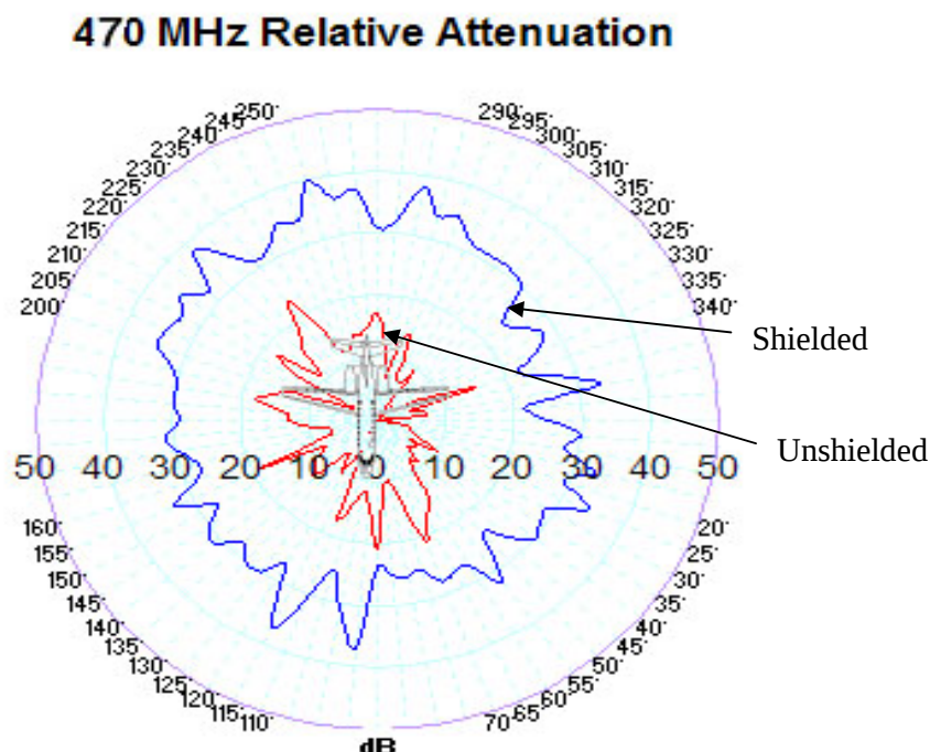
Figure 16. Relative attenuation Shielded Vs Unshielded 470 MHz
