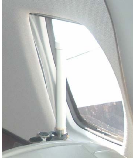
Figure 10. Typical inside PCS antenna location for ingress testing
