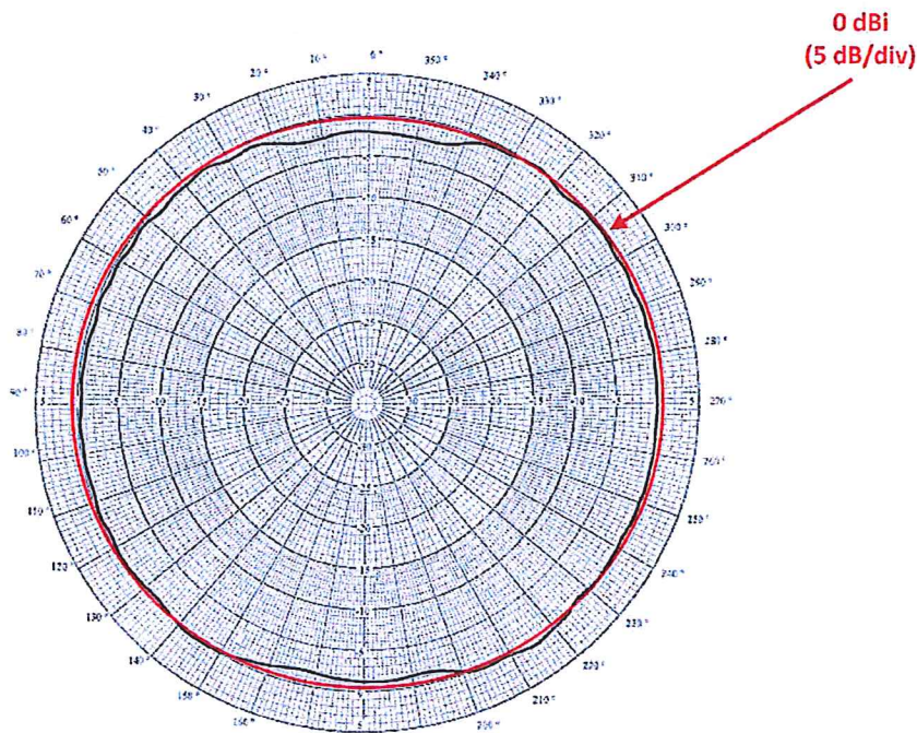
AZIMUTH (YAW) 2.250 GHz
