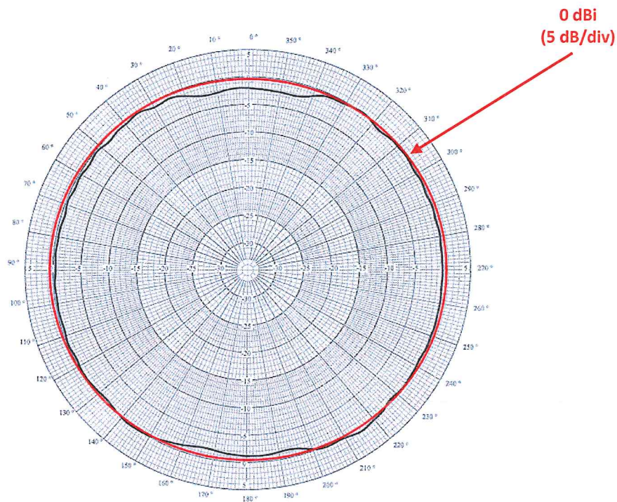
AZIMUTH (YAW) 2.250 GHz
