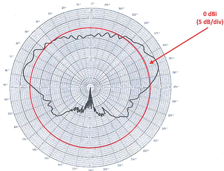
ELEVATION (PITCH) 2.250 GHz
