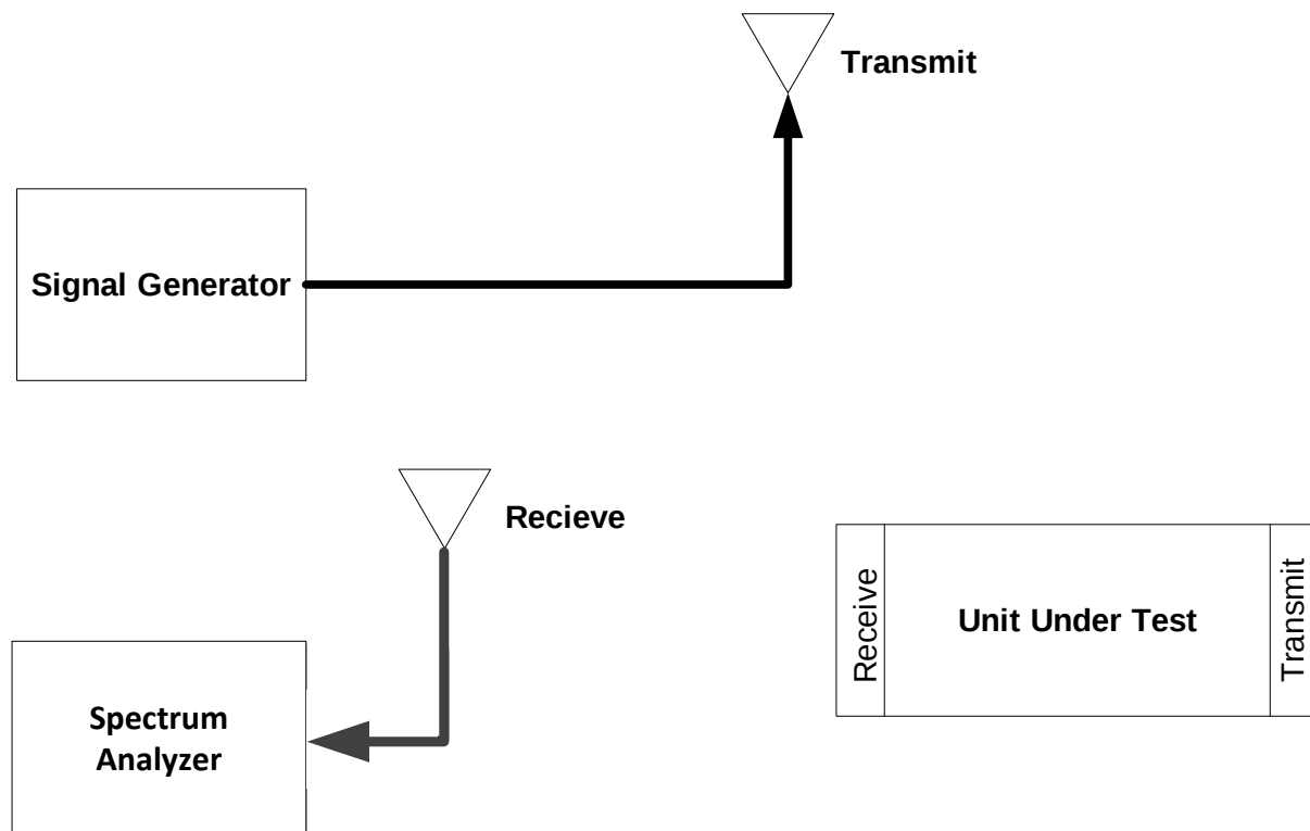
Figure 1. Isolation Margin Test
