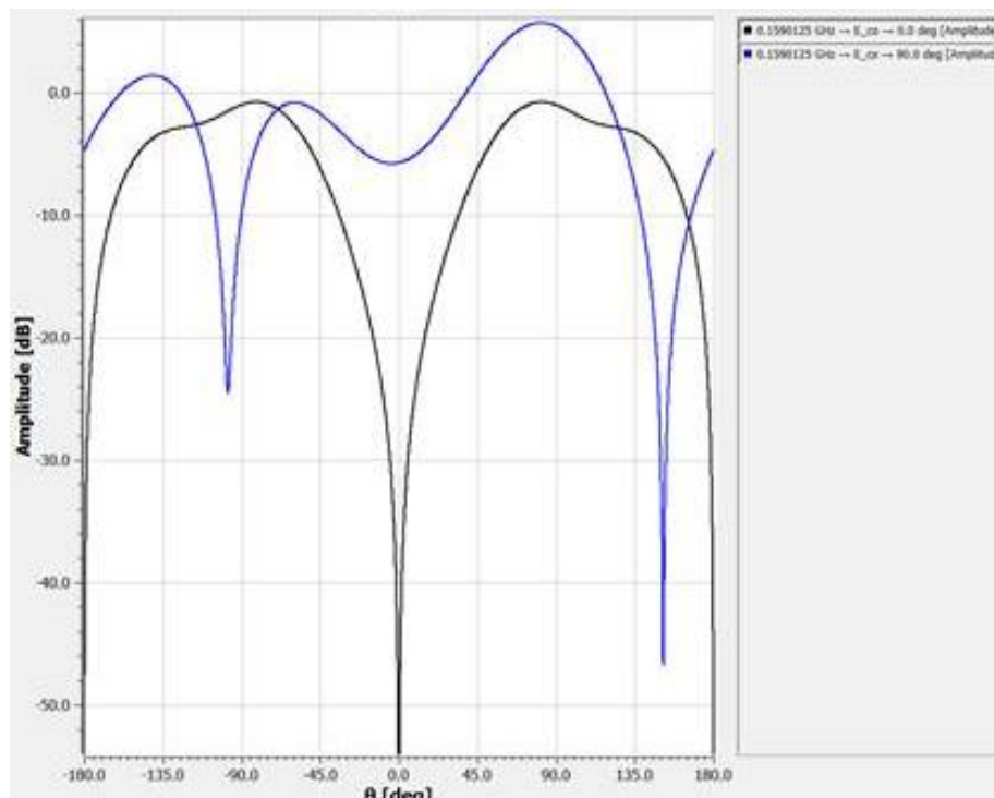
Figure 2-7: AIS Monopole Antenna Directivity
