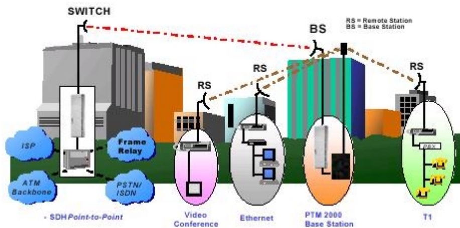
Typical representation of PTM 2000 in a Broadband Wireless Access Network
