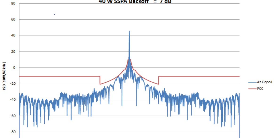
MUAP Predicted ESD: Copol/Az/27.652 GHz Max Copol EIRP = 45.761 dBW/4kHz 40 W SSPA Backoff = 7 dB
