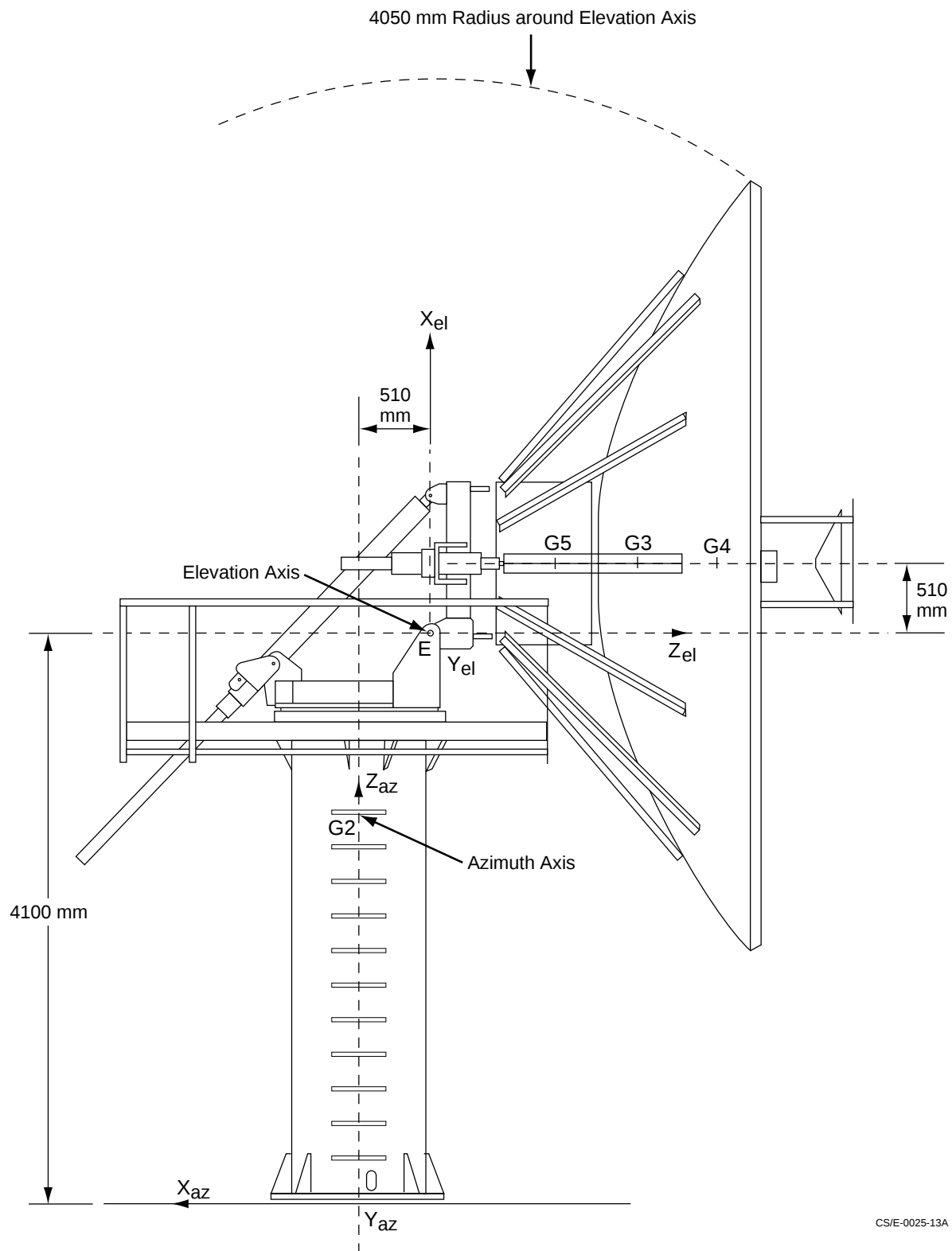
Figure 3-3 ALCATEL Antenna Subsystem Side View (4/26/96)
