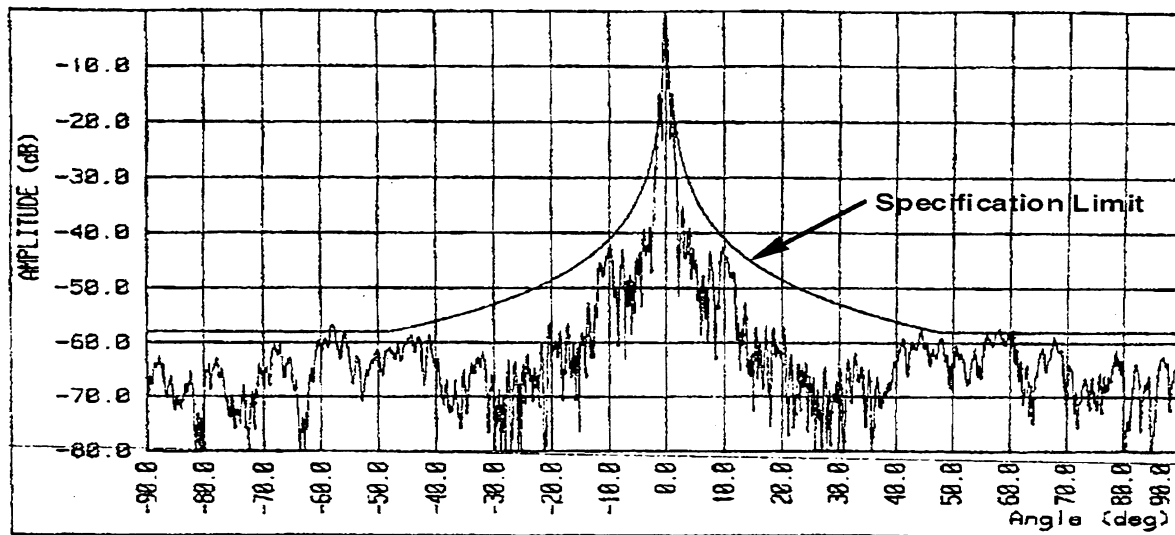
Antenna gain versus off pointing angle Alcatel M/N 9775 5.5 m Parabolic Antenna
