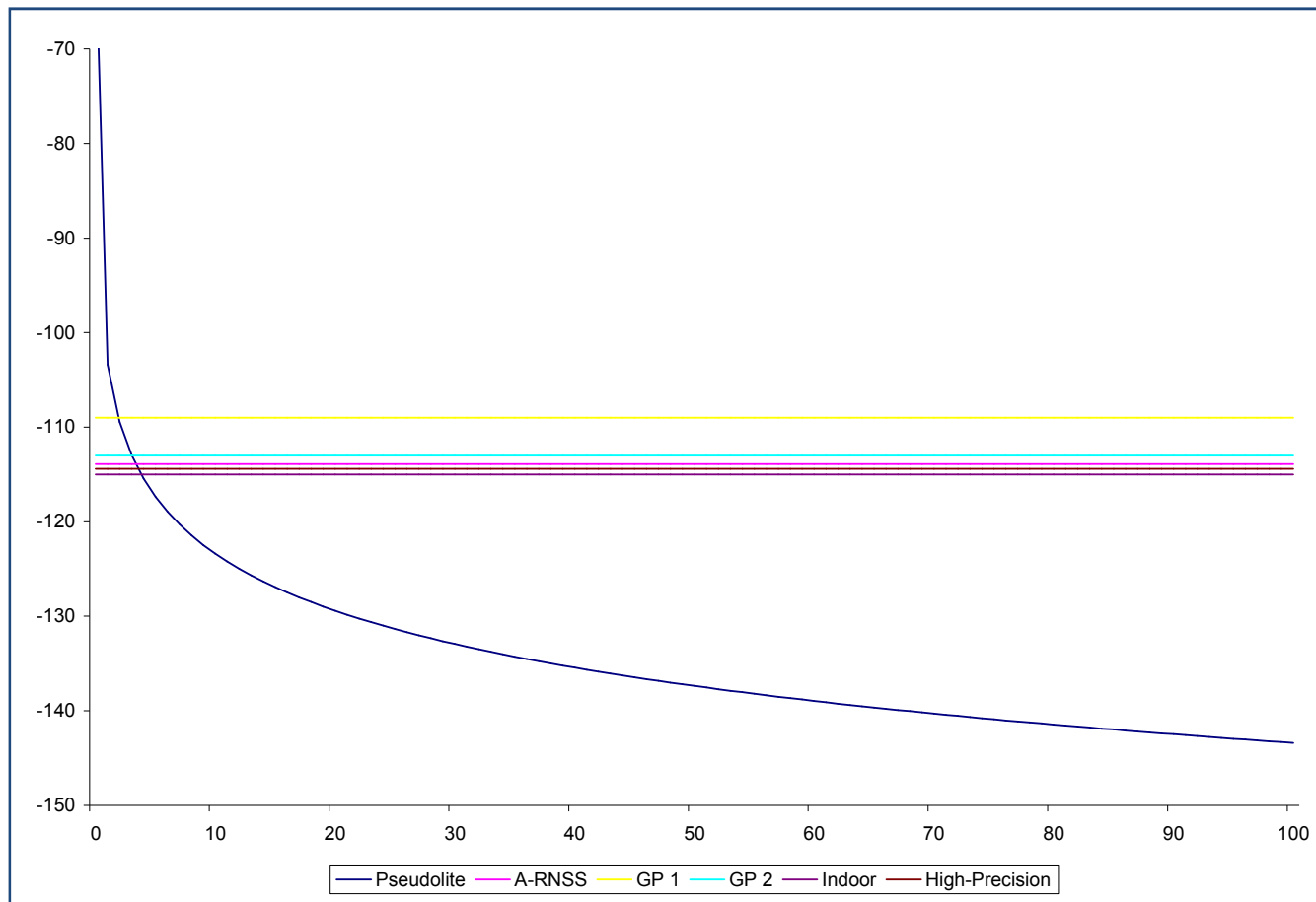
FIGURE 1: PSEUDOLITE POWER OVER DISTANCE V. INTERFERENCE THRESHOLDS OF NON-PARTICIPATING RECEIVERS (CURVED LINE REPRESENTS PSEUDOLITE POWER PROFILE AT VARIOUS DISTANCES)
