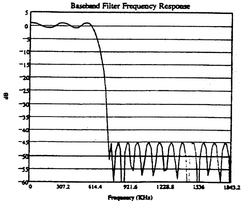
Baseband Filter Frequency Response
