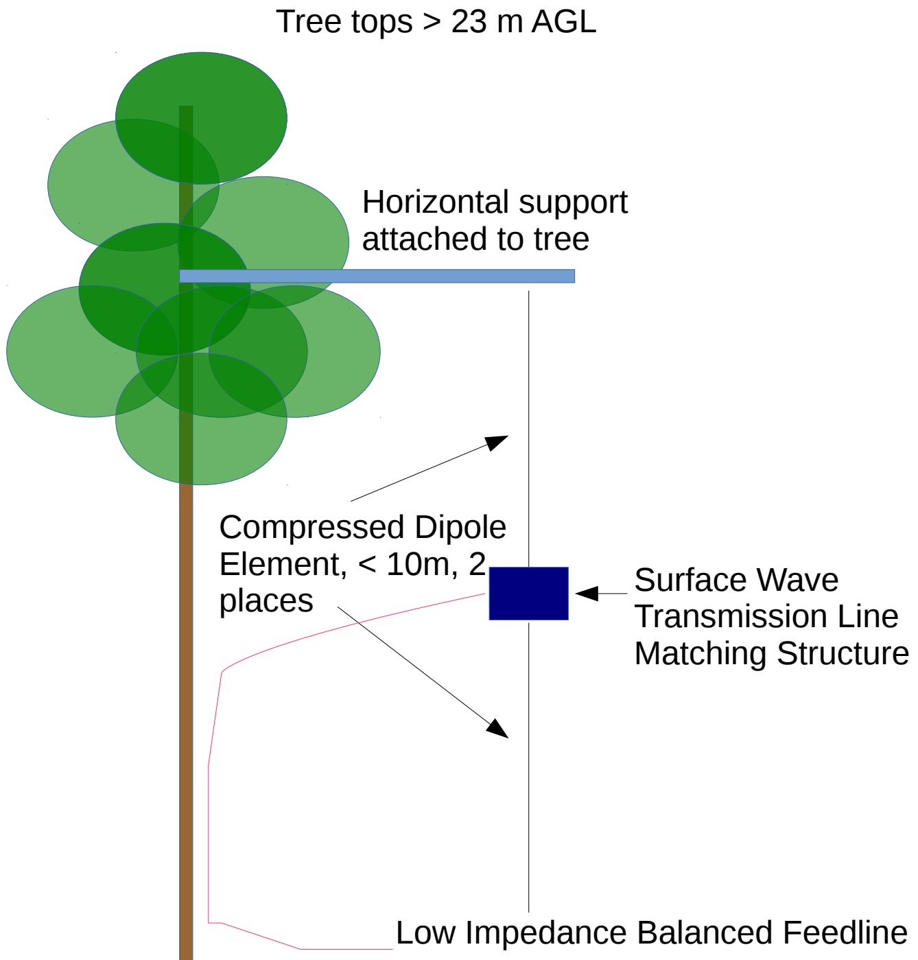
Sketch of 446 Halter Court, 137 and 475 kHz Compressed Dipole Experimental Antenna
