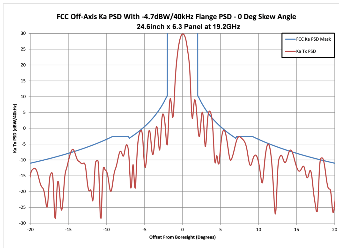
Figure 2 Transmit PSD
