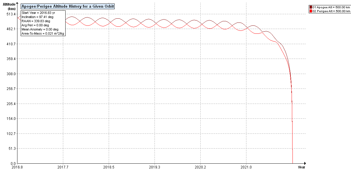
Figure 7: RANGE orbit history for high-drag configuration
