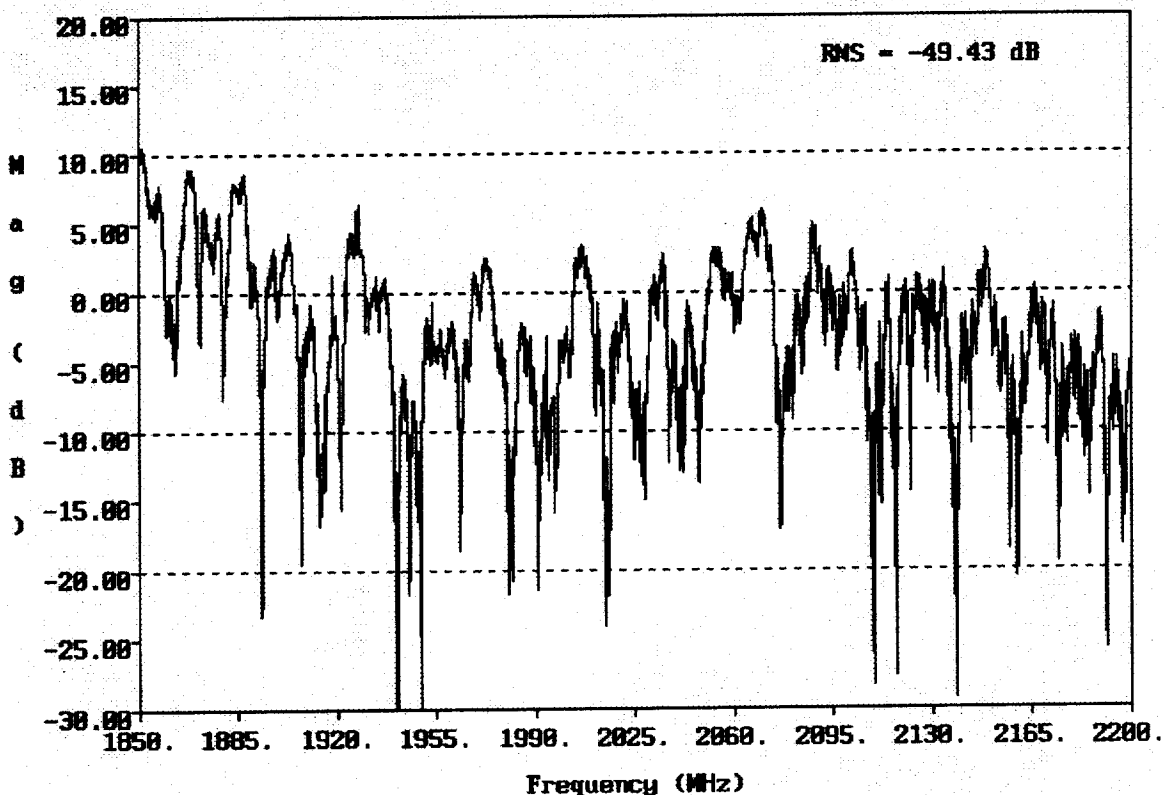
Figure 4-3 Log Magnitude Frequency Response of Cross Courtyard Channel.
