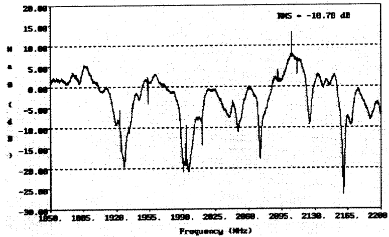
Figure 4-4 Log Magnitude Frequency Domain Data, 1 cm Fine Grain Linear Series
