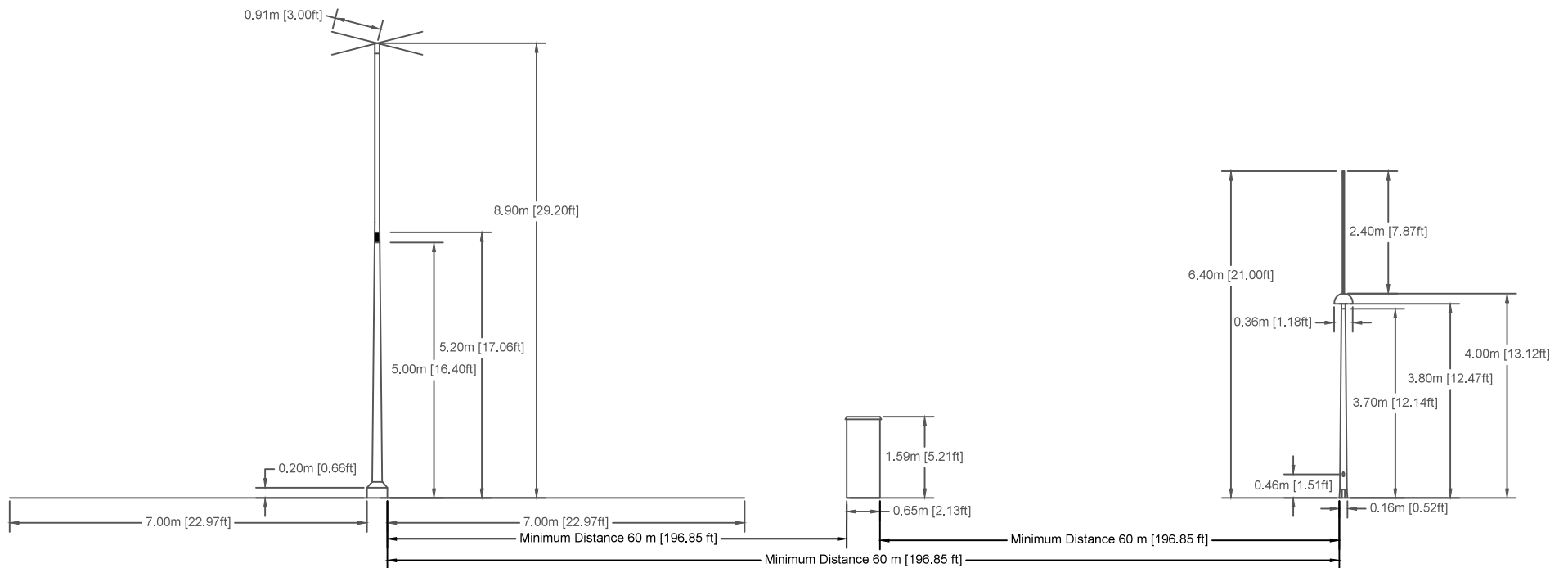
Transmit Antenna
