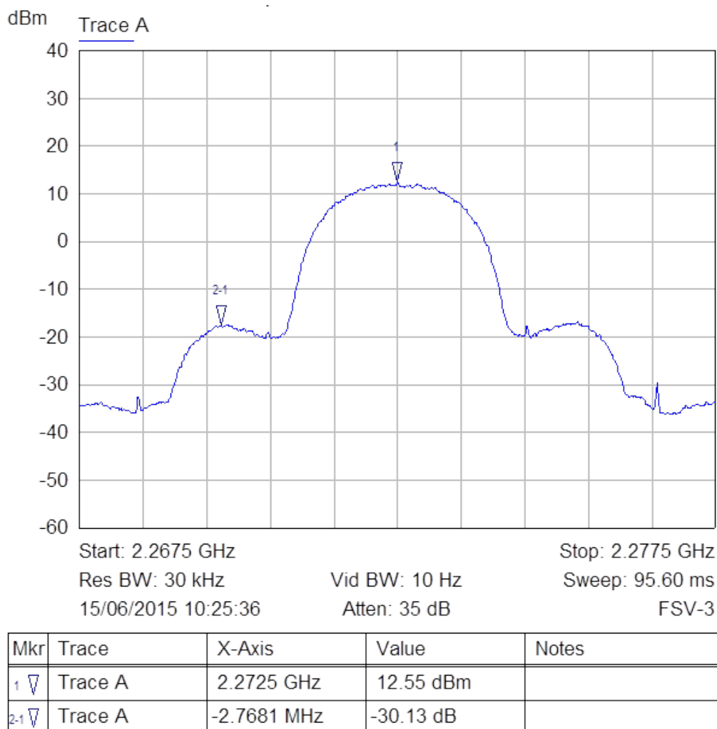
Figure 6-2: Emission spectrum of S-Band High Rate Tx
