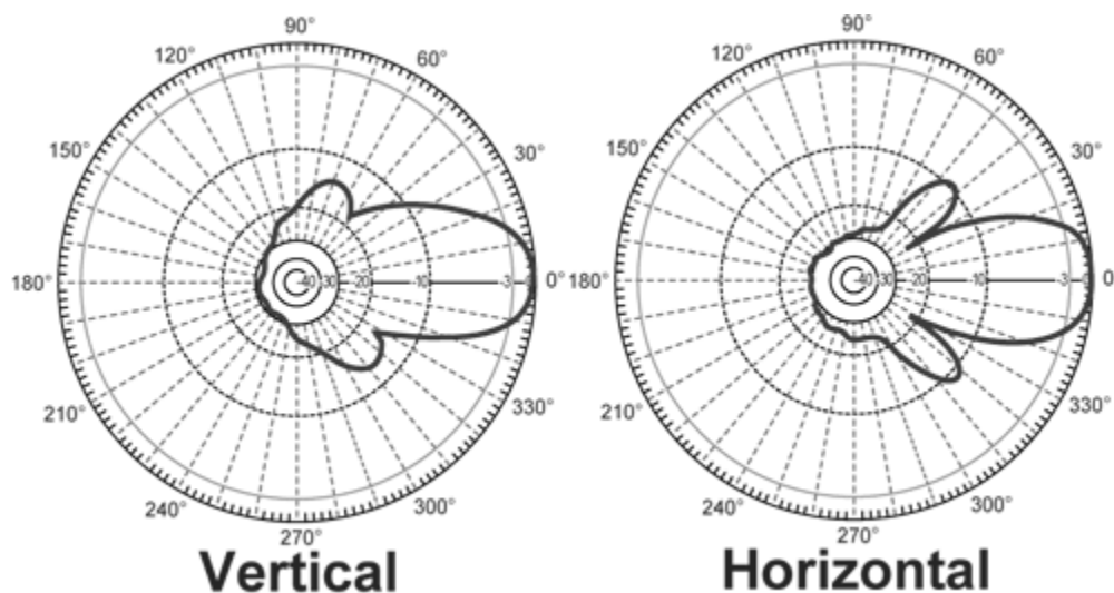
Figure 1 - HG5817D Antenna Gain Patterns
