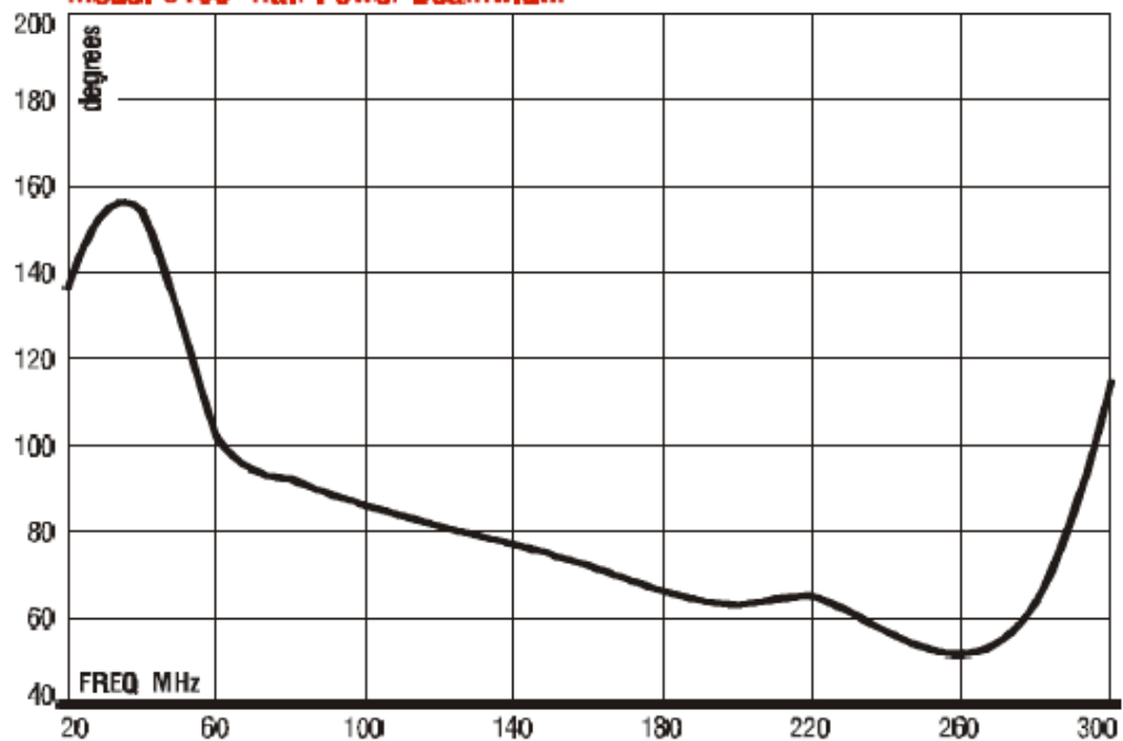
Model 3109 Half Power Beamwidth
