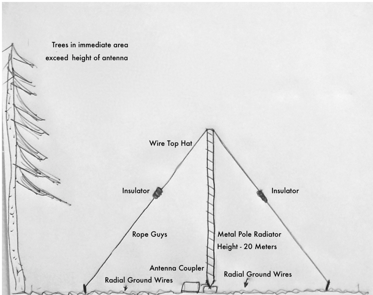
Antenna Diagram
