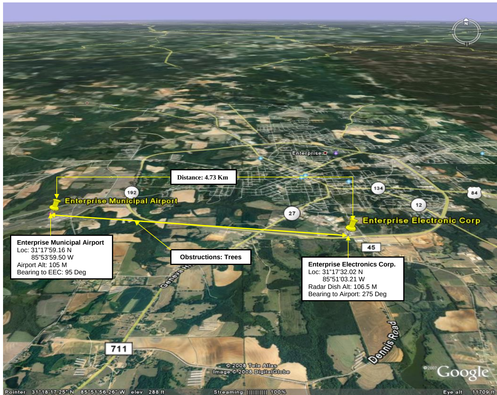
FAA Antenna Sketch Diagram
