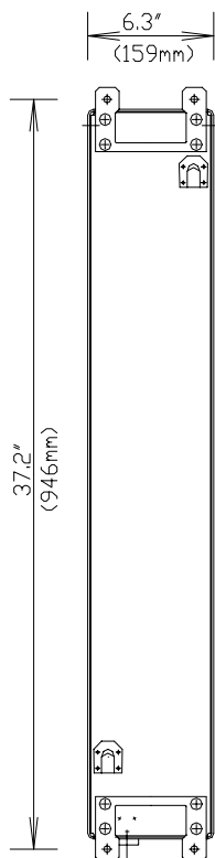
REAR VIEW
