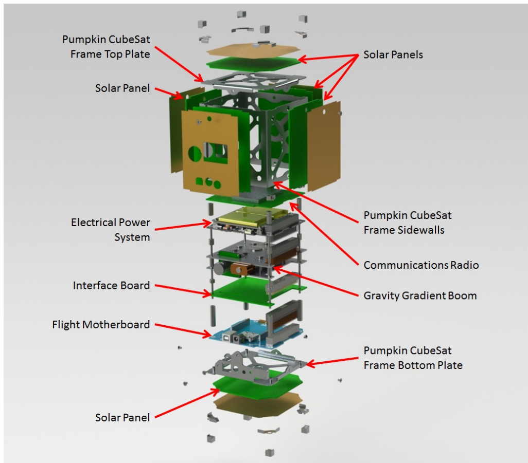
Figure 2: DragonSat-1 Expanded View
