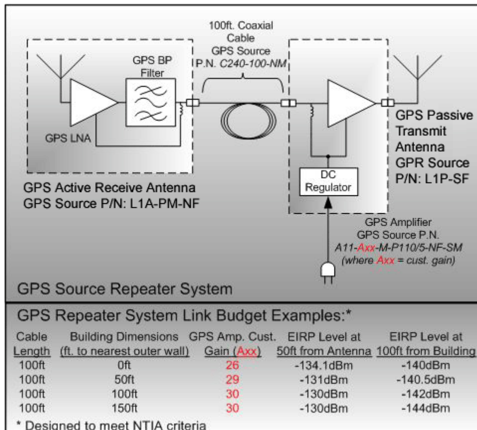
Figure 1. GPS Source typical Repeater System
