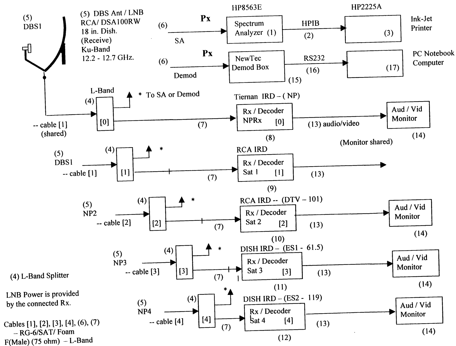
Fig. II-3: Mobile Receiver System Block Diagram
