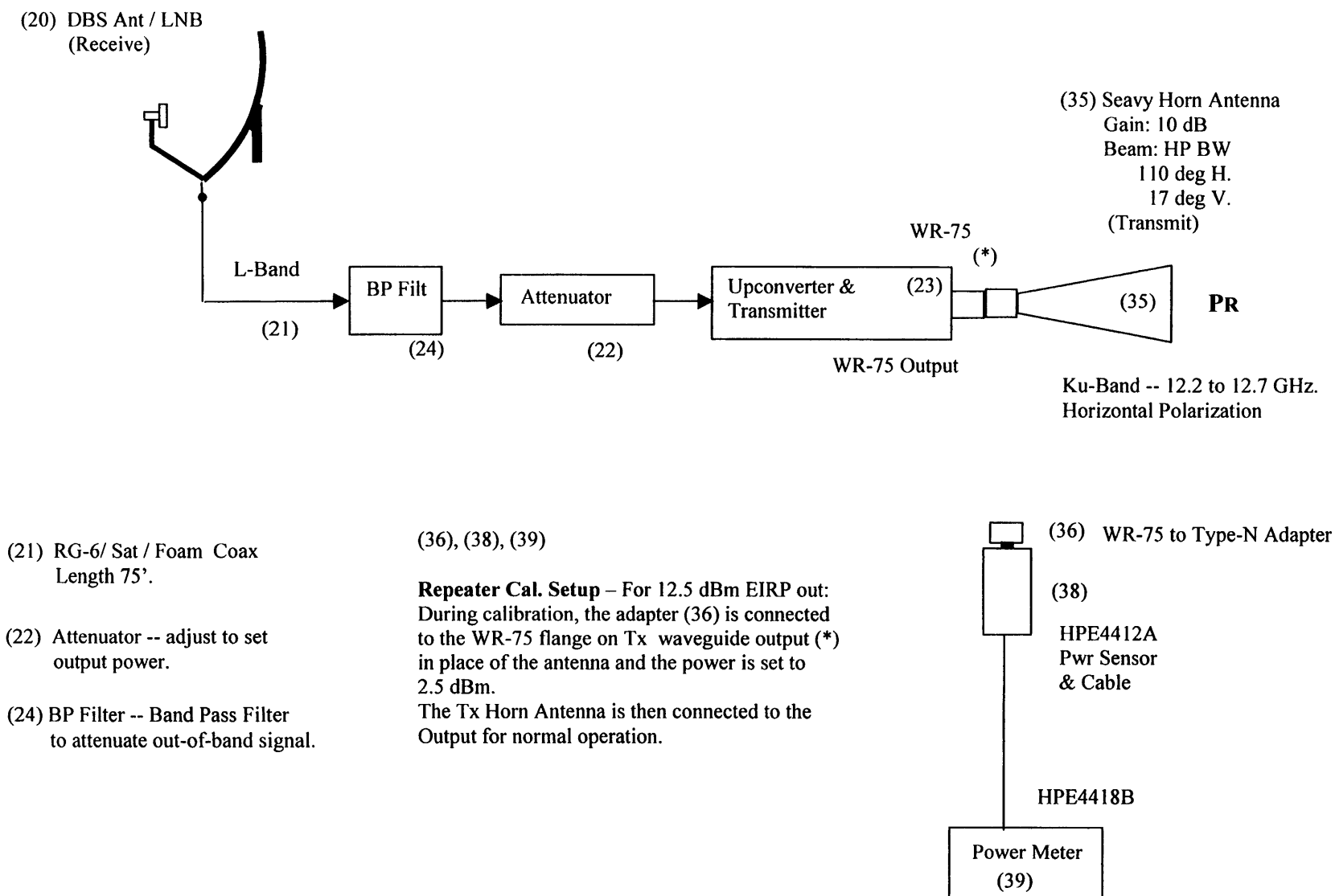
Fig. II-2: Northpoint Terrestrial Repeater Block Diagram.
