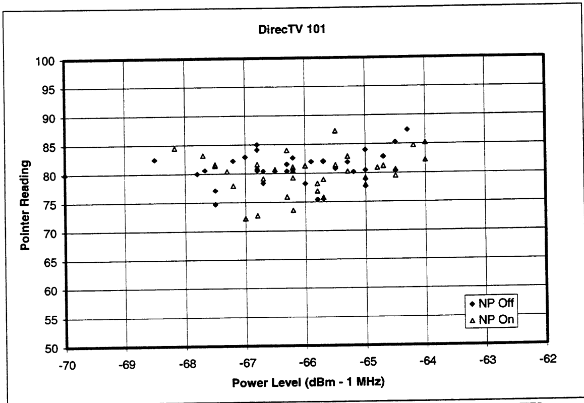
Figure 2. Plot of Pointer Reading vs. Power Density Level for DirecTV
