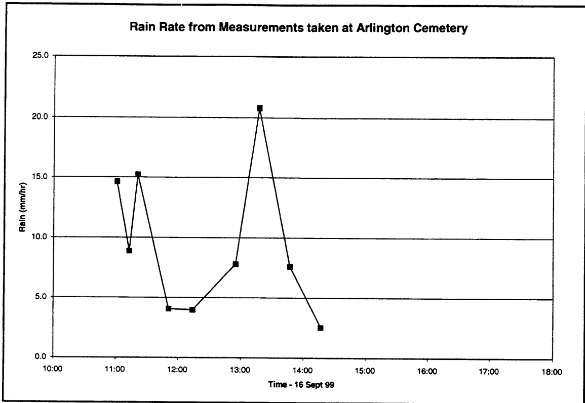
Figure 10. Rain Rates from Measurements taken at Arlington Cemetery
