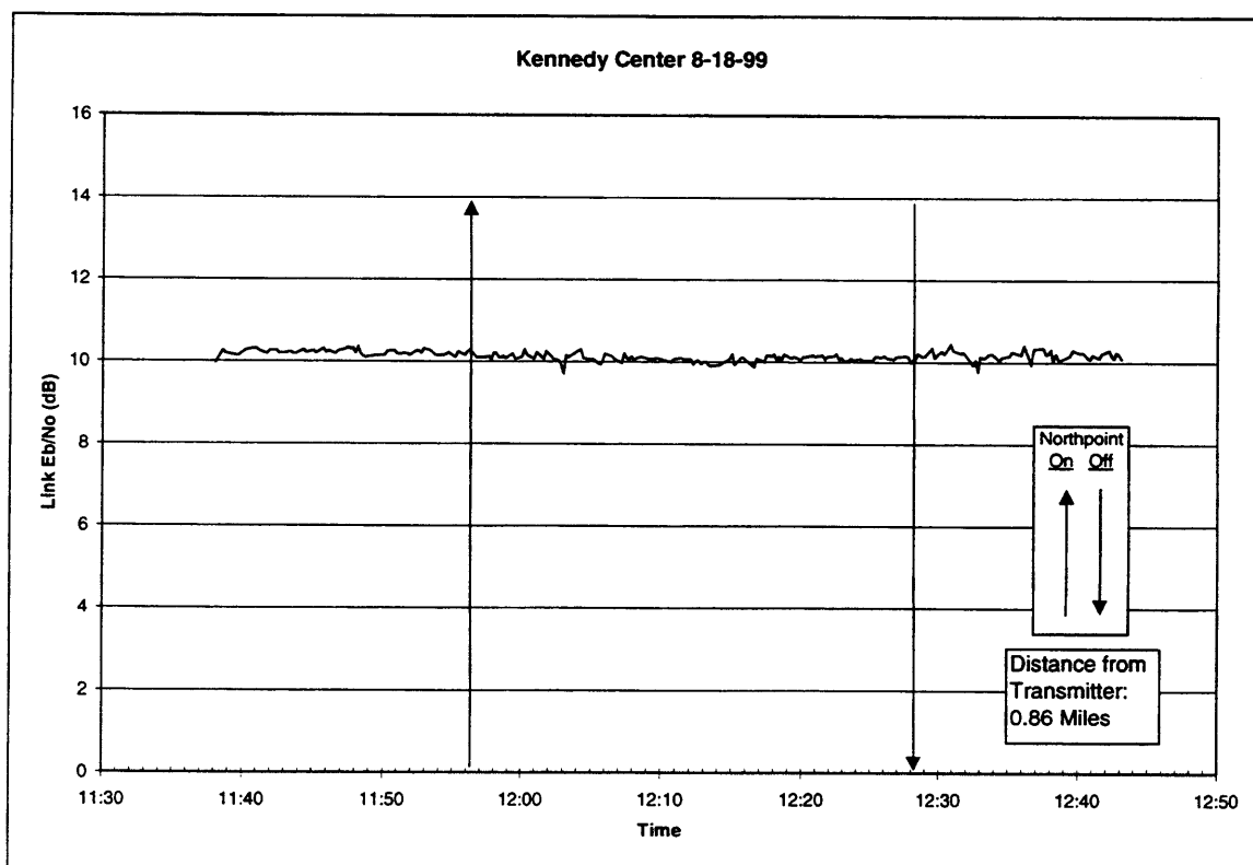
Figure 8. Link Degradation for Echostar 119, Kennedy Center
