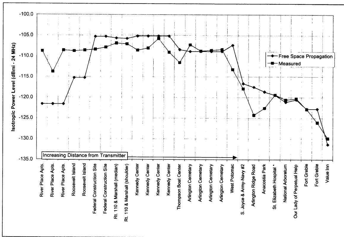
Figure 15. Northpoint Signal Strength
