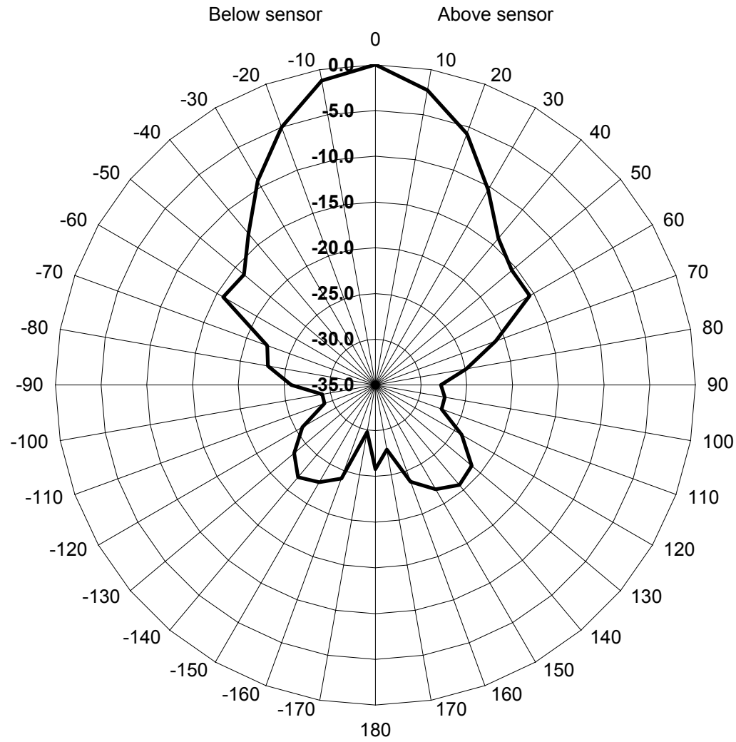
QUPID Far Field (29 meter) Elevation Plot
