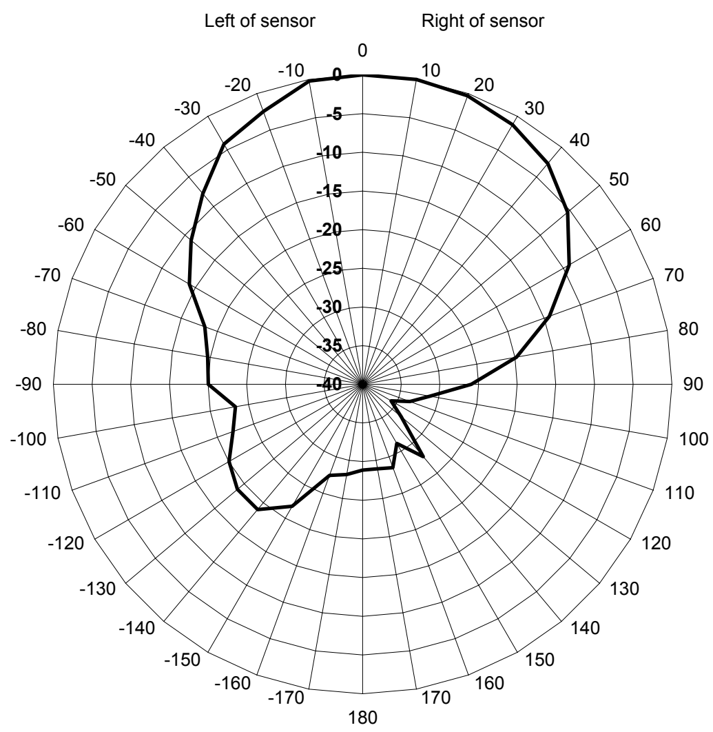
QUPID Far Field (29 meter) Azimuth Plot
