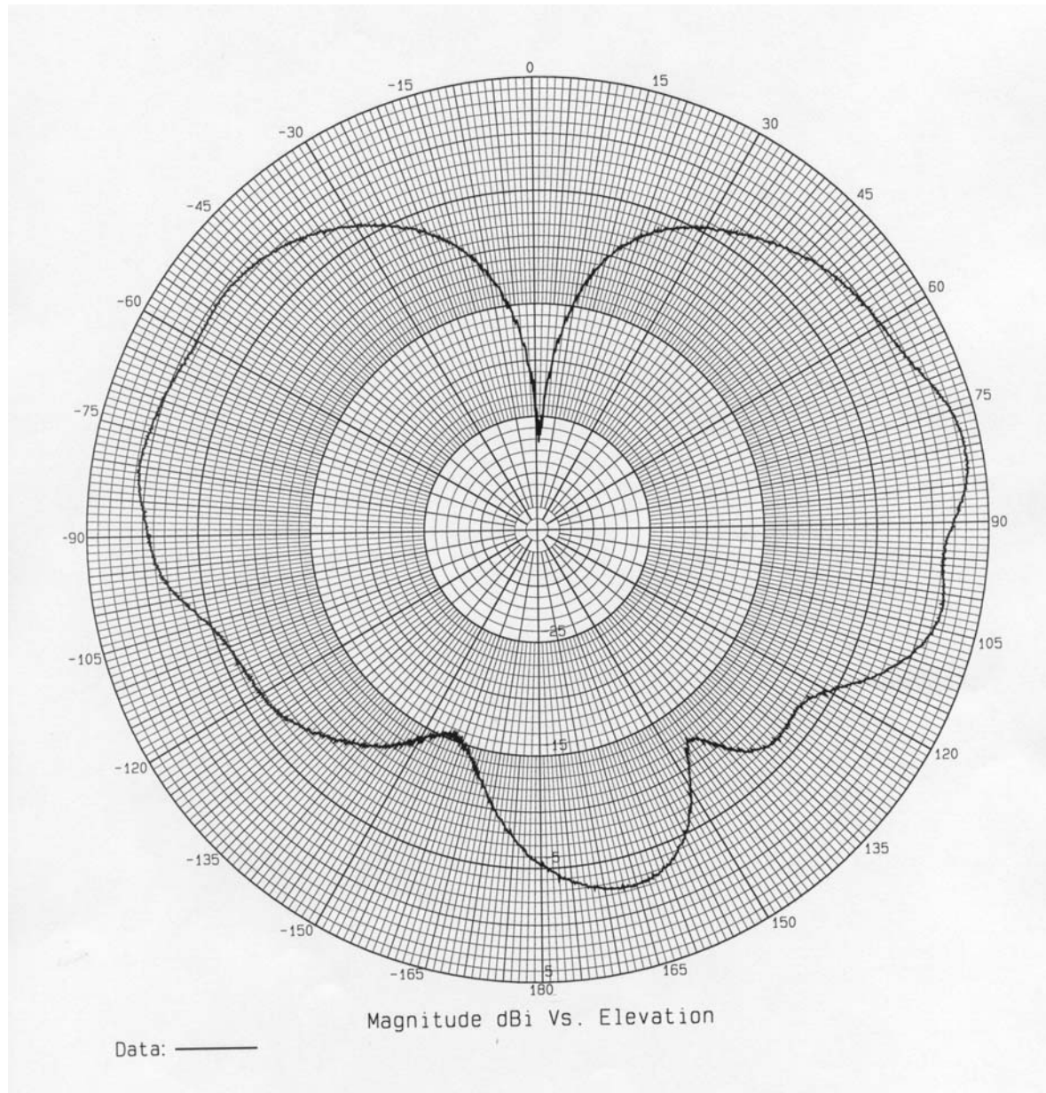
PSTN2-4500 Series – Elevation Plot
