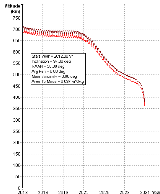
Figure 3: Dove 4 (right) orbit history with apogee (brown) & perigee (red) plotted.
