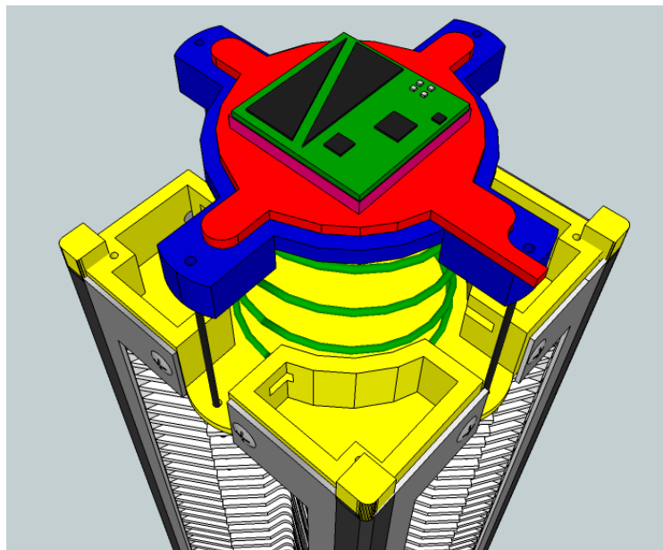
Figure 3: KickSat Deployment
