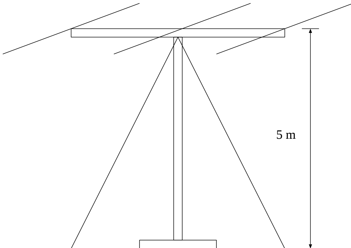
Figure 1: Diagram of one of the antennas used for our research project. The antennas are three-element yagis atop temporary poles supported by guy wires. They are modified versions of amateur-radio antennas (Hy-Gain LJ-103b). Eight such antennas in a line form an array with a main beam directed toward Puerto Rico.
