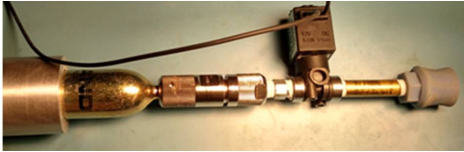
Figure 14: Cold Gas Thruster Assembly
