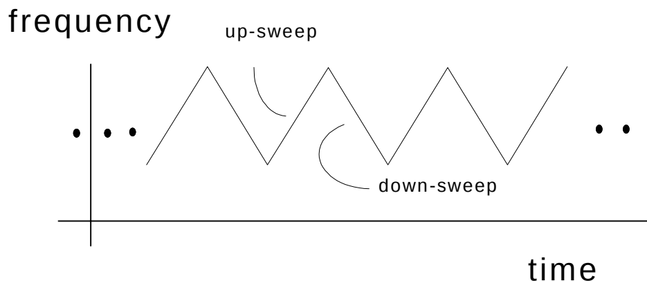
Figure A.3 - Actual Signal is Continuous Constant-Envelope Repetitive Linear FM Sweep Signal Having Rectangular Power Spectrum
