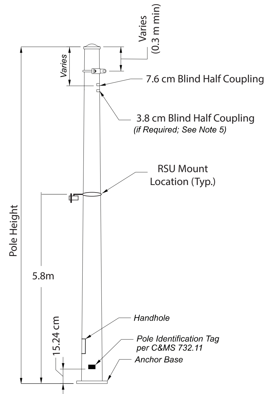
Strain Pole Installation Detail Not to Scale
