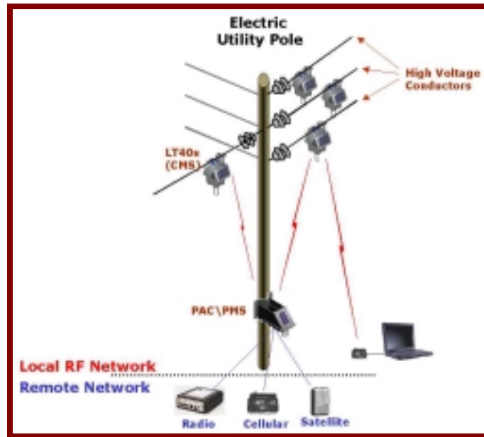
Figure 1. Typical LT40 Installation.
