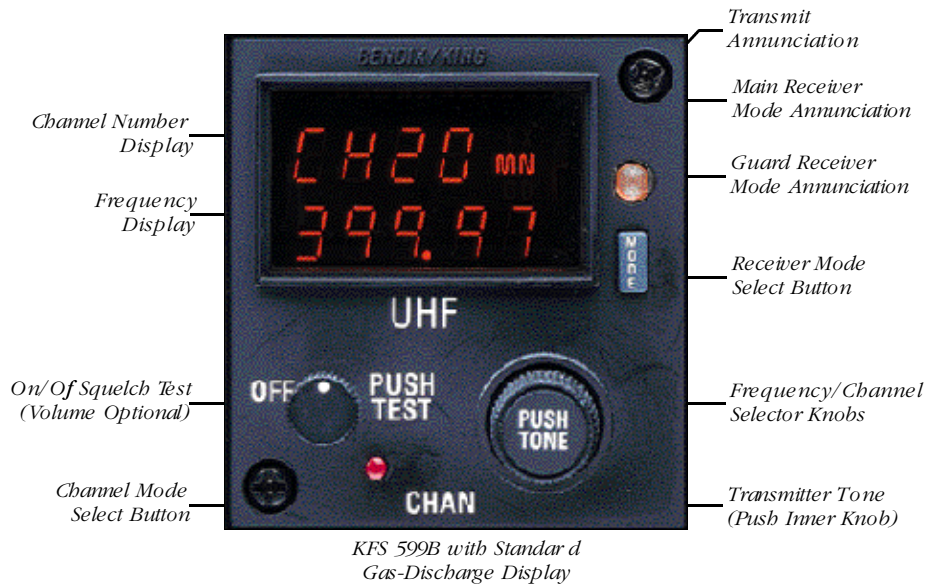
The KTR 909B is controlled via the KFS 599B control head (shown above), which supports the ARINC 429 interface. The KTR 909 uses either the standard KFS 599A control head or an available NVG-compatible variant.
