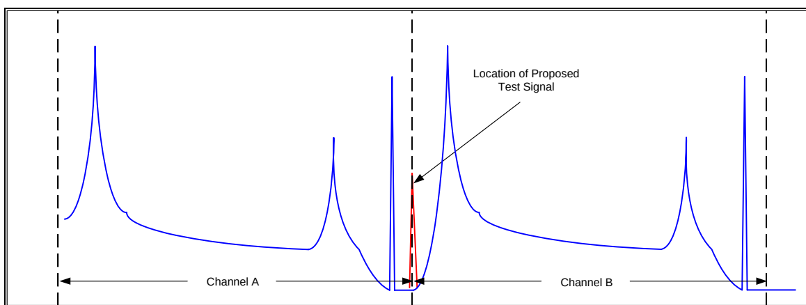
Fig. 2 - Location of Proposed Signal Relative to NTSC Channel Spectrum
