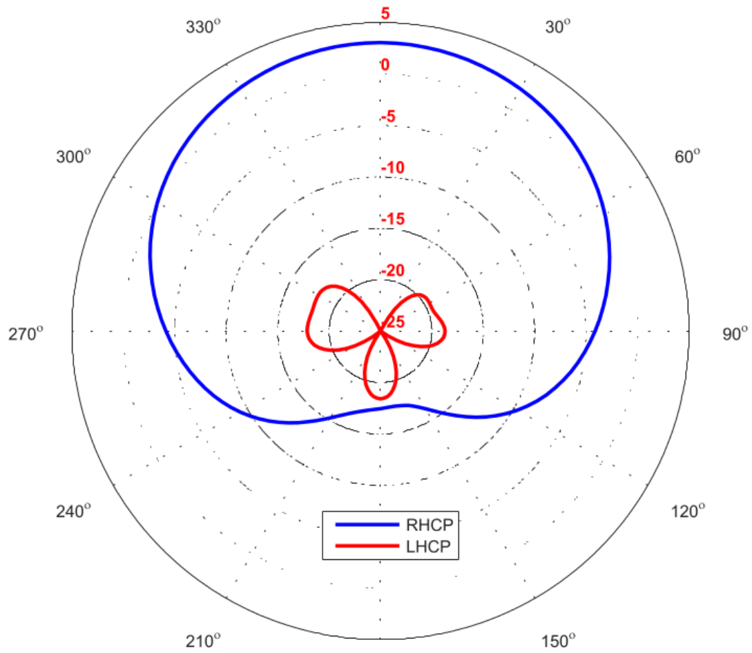
IRIDIUM Antenna Radiation Pattern Diagram
