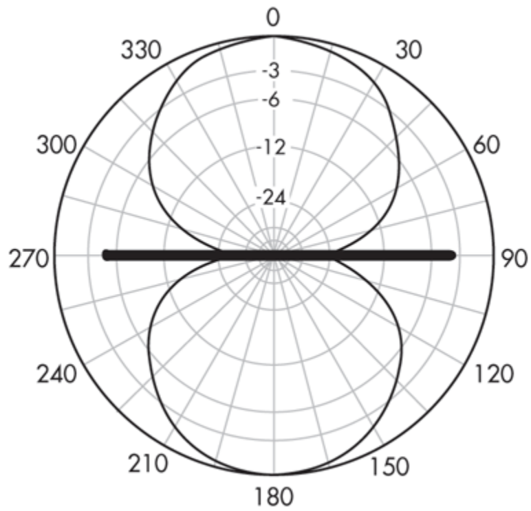
Satellite Dipole Antenna Radiation Pattern Diagram
