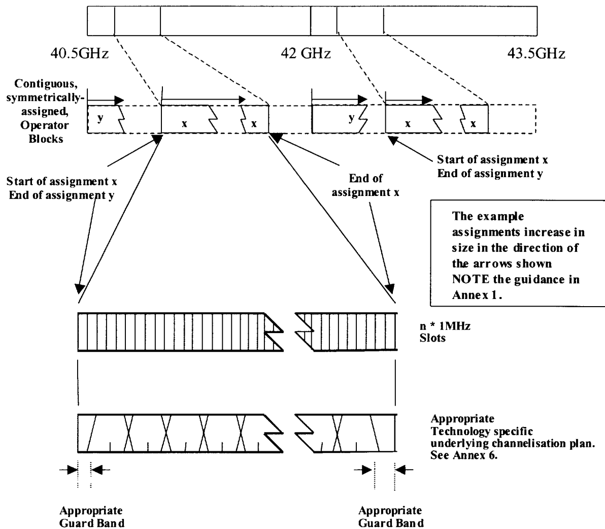
Figure 3.1: Frequency Plan Elements
