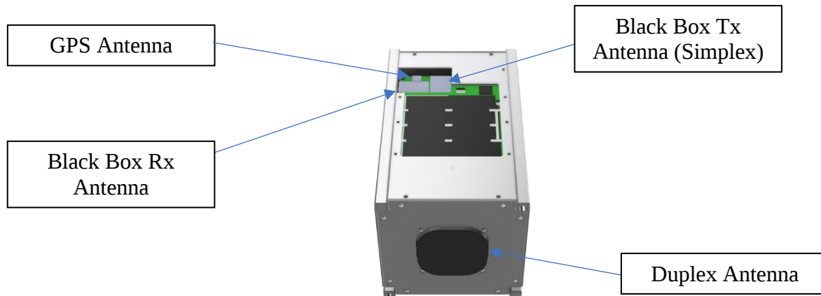
Figure 1 BroncoSat-1 Overview
