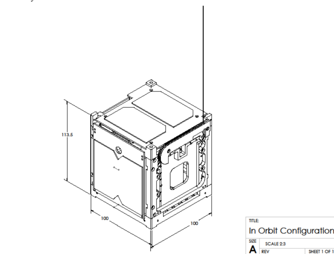
Figure 2: IPEX Dimensions
